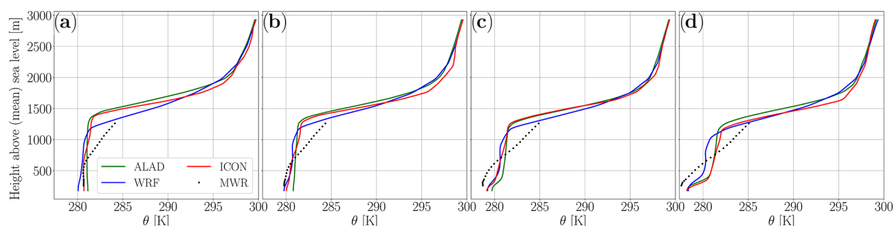
Figure 5. (a–d) Comparison of the potential temperature ( \Theta ) profiles modeled by the mesoscale models ICON (red), ALADIN (green), and WRF (blue) used as PALM model BCs with profiles from MWR observations (dots). The displayed hours cover the concentration peak of 13 February: 16:00 (a), 17:00 (b), 18:00 (c), and 19:00 (d). Values represent hourly averages for the hour ending at the given time.
