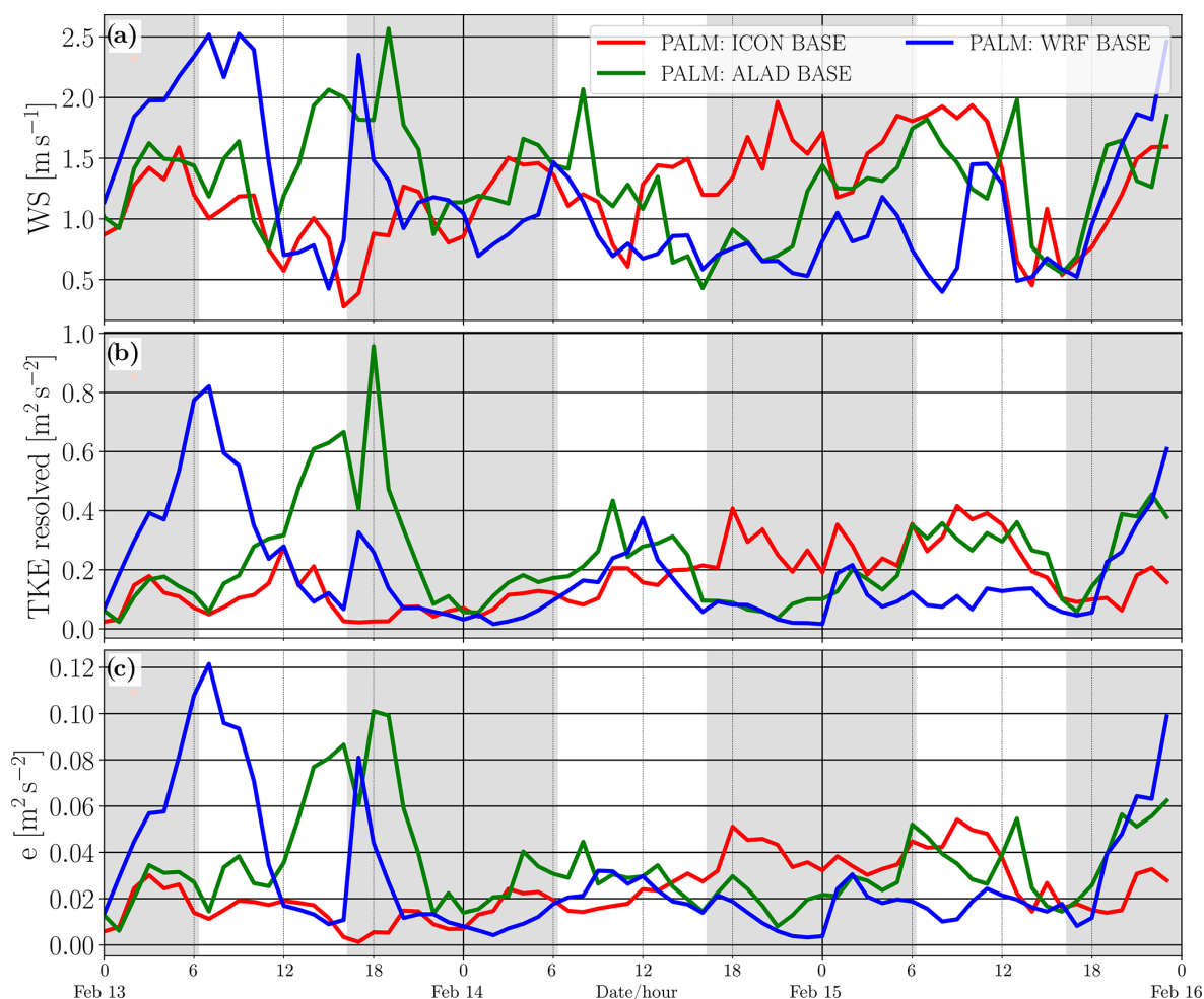
Figure 8. (a–c) Comparison of the PALM-modeled wind speed (WS), resolved TKE (TKE), and SGS TKE (e) at the location of the ALEGA AIM station for scenarios PALM-ICON (red, base case), PALM-ALAD (green), and PALM-WRF (blue). The gray areas represent nighttime, and white areas represent the daytime.
