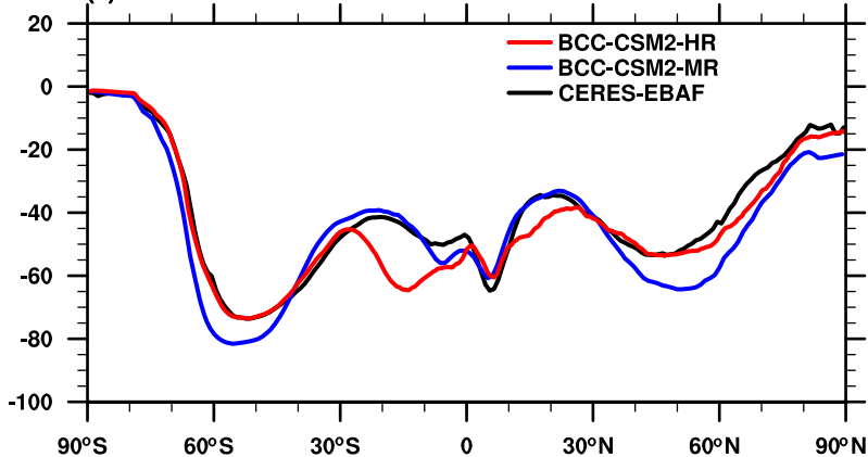
(a) Shortwave CRF
