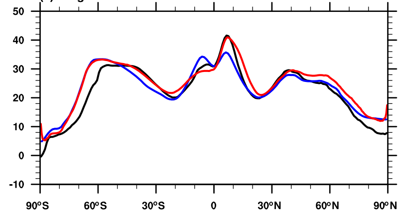
(b) Longwave CRF
