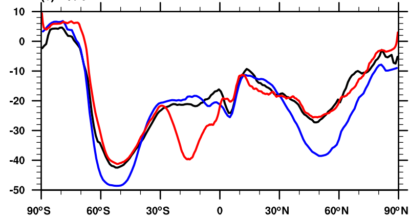
(c) Net CRF
