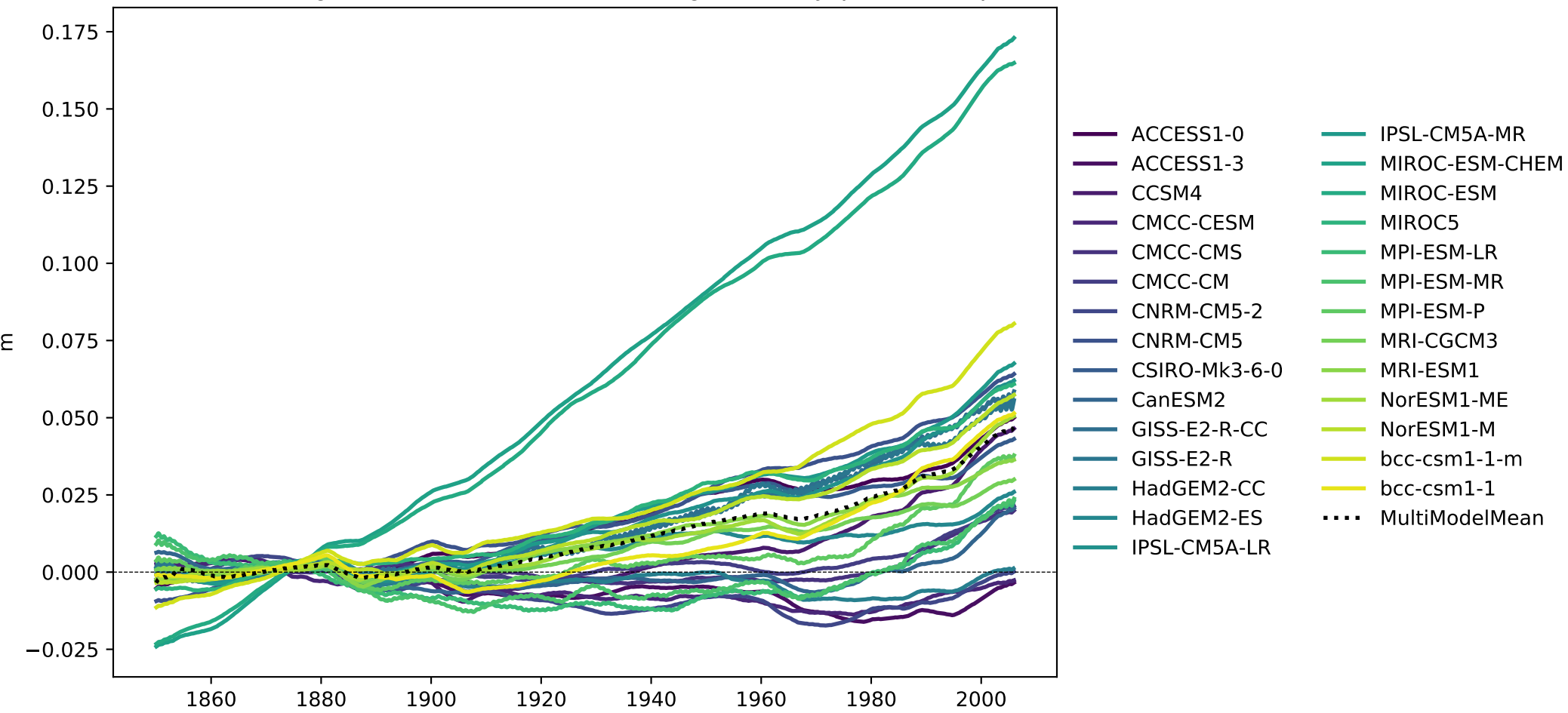
Global average thermosteric sea level change anomaly (1850–1900)
